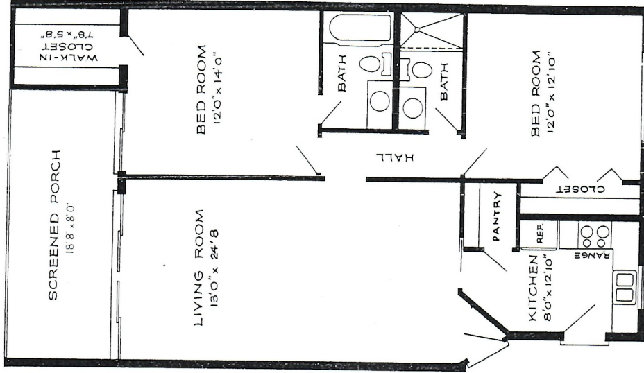
FLOOR PLAN "B"
